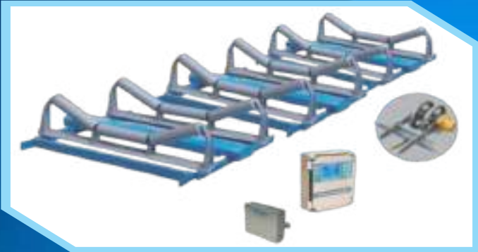
Belt Scale System 4 Loadcell
